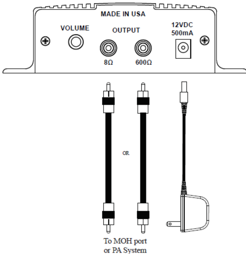
Wiring Diagram
