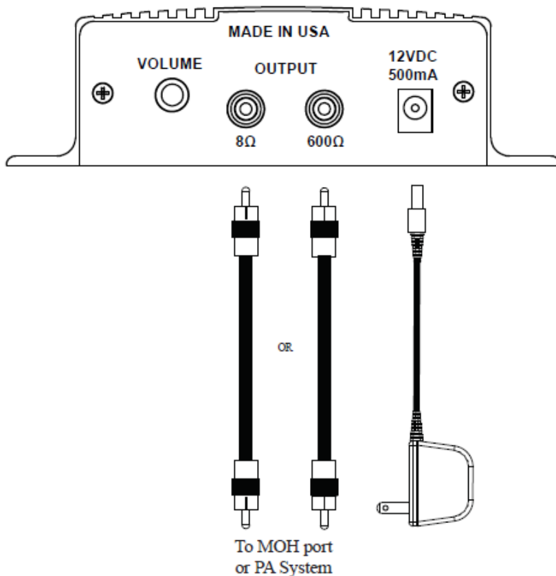
Wiring Diagram
